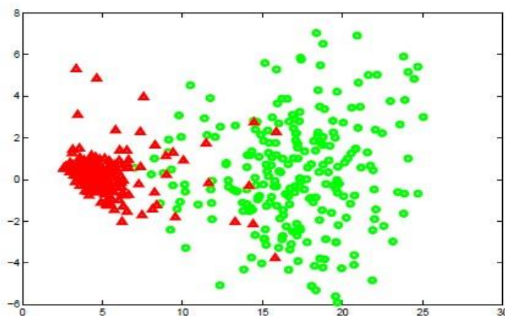
Fisher Discriminant Analysis – FDA
