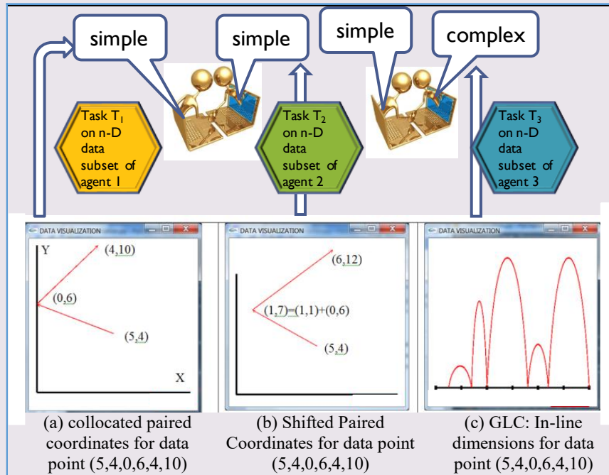
Collaboration diagram with data example 1.
