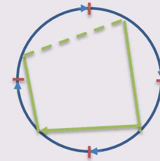
(b) Circular Coordinates display.
