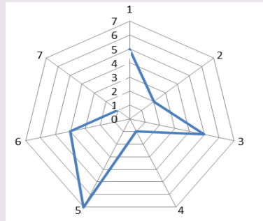
7-D point D=(5,2,5,1,7,4,1) in Radial Coordinates.
