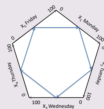
(b) Example in n-Gon coordinates with straight edges of a graph.
