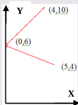
(a) Collocated Paired Coordinates.
