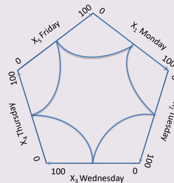
(a) Example in n-Gon coordinates with curvilinear edges of a graph.
