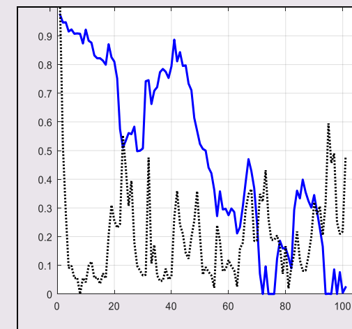
Comparison of two time series: relative outcome Y_r and relative volume in every one hundred period.
