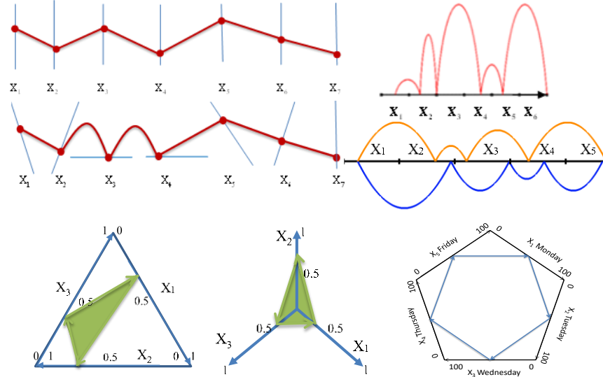
Fig. 9. Examples of different GLCs: Parallel, Non-parallel, Curved, In-line Coordinates Pentagon, Triangular, and Radial Coordinates.
