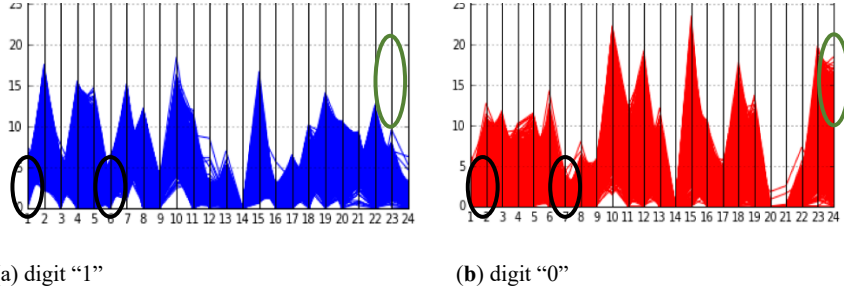
Fig.20. Comparing encoded digit 0 and digit 1 on the parallel coordinates using 24 dimensions found by the Autoencoder among 484 dimensions. Each vertical line is one of the 24 dimensions.
