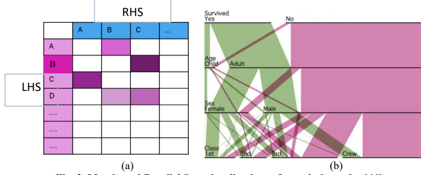
Fig. 3. Matrix and Parallel Sets visualizations of association rules [46].
