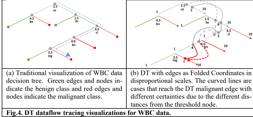
Fig.4. DT dataflow tracing visualizations for WBC data.
