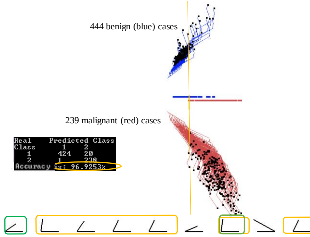
Fig. 11 GLC-L WBC data example.
