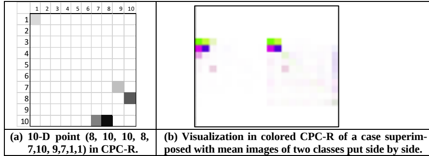
Fig. 17. CPC-R visualization of non-image 10-D points.
