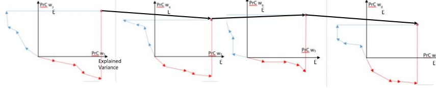
Fig. 21. All PCA principal components w_1 - w_8 , visualized in Shifted Paired Coordinates, and GLC-Linear coordinates, for an 8-D data point x=(x_1, x_2, \dots, x_8) , without loss of information.
