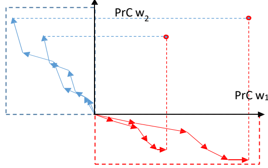
Fig.22. Two 4-D points in the first two principal components in GLC-PCA.
