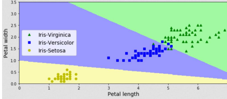
Fig. 2. Example of logistic regression classification of Iris classes [3].
